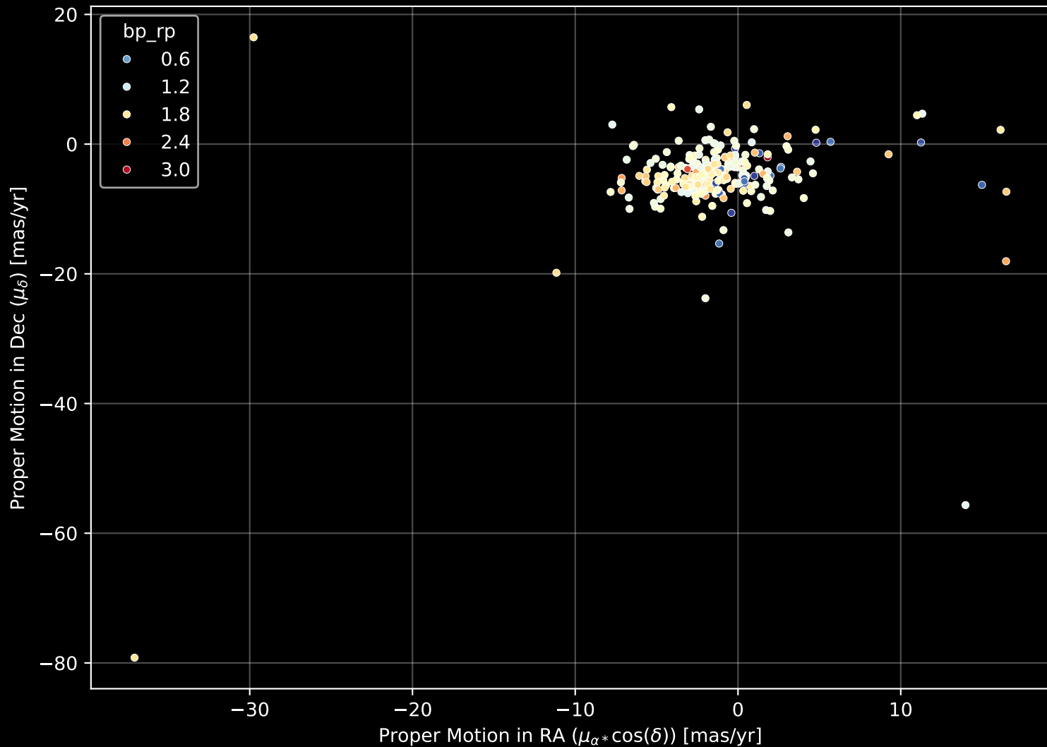
APOGEE DR17 Field: [025-12] Proper Motion Diagram (n= 254)
