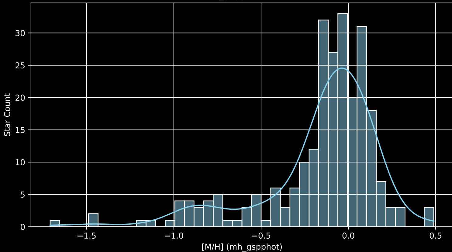
APOGEE DR17 Field: [025-12 [M/H] (mh_gspphot) (n= 251)
