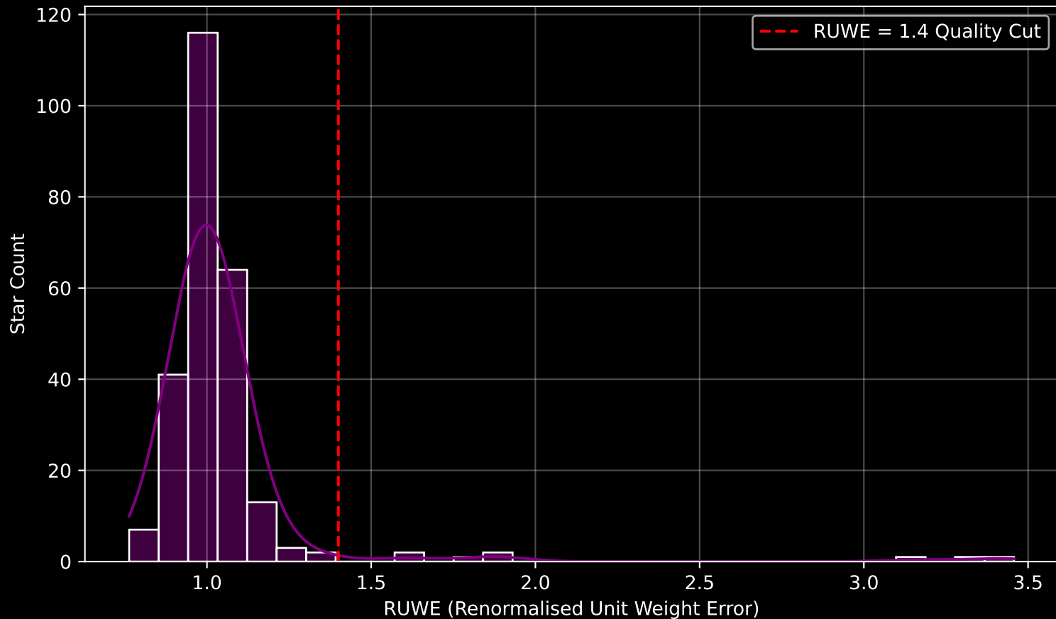
GAPOGEE DR17 Field [025-12] RUWE Distribution (n= 254)
