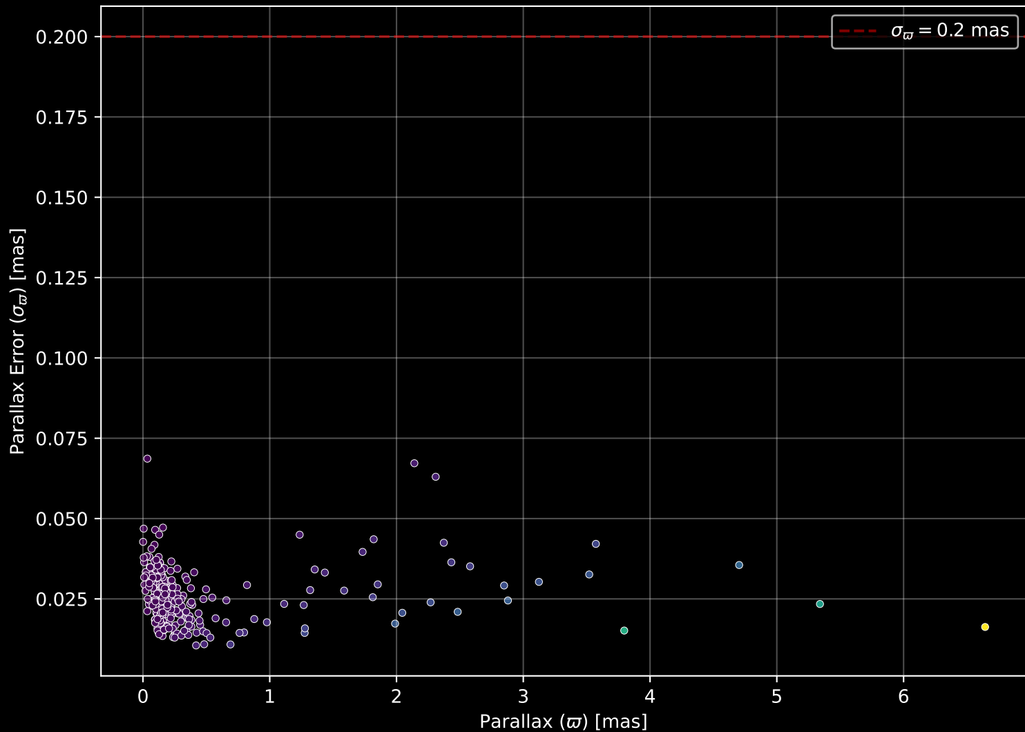
APOGEE DR17 Field: [025-12] Parallax Quality (n= 254)
